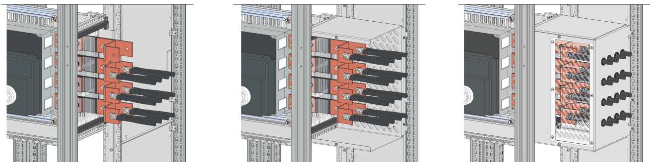
Conductor Connections from MCCB Output to Terminal .
